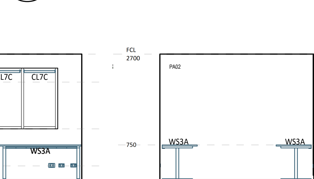
13 ELEVATION DETAIL 60-13 1:50
