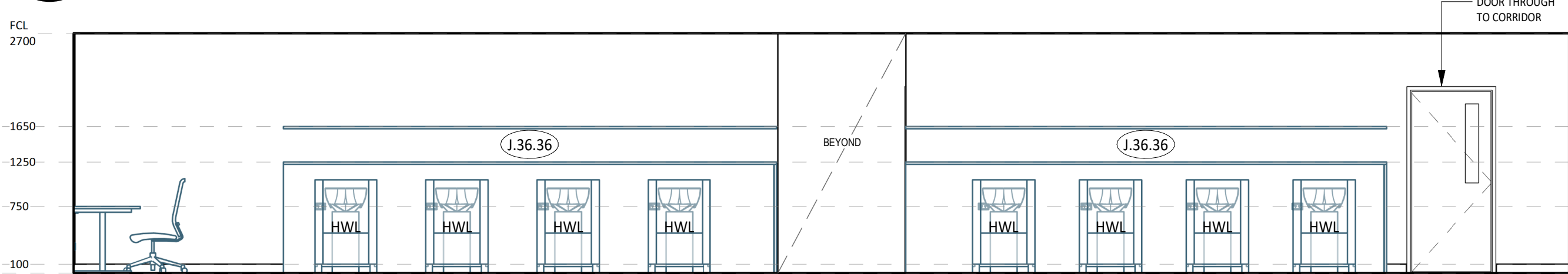
5 ELEVATION DETAIL 60-13 1:50
