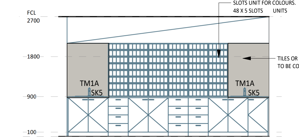
7 ELEVATION DETAIL 60-13 1:50
