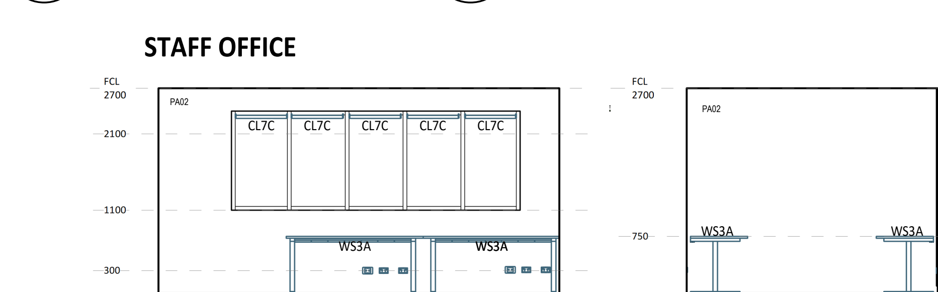
12 ELEVATION DETAIL 60-13 1:50
