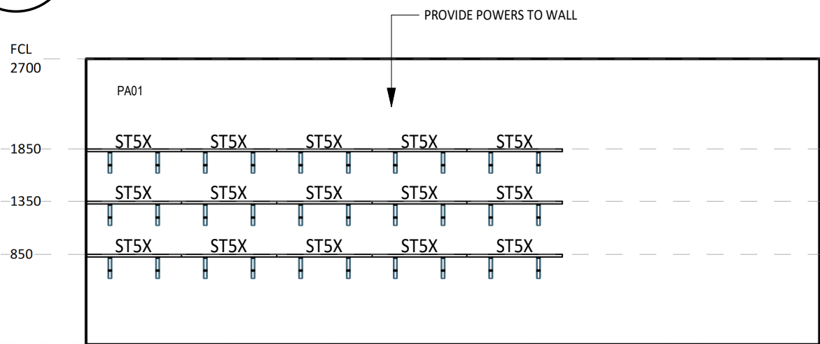
10 ELEVATION DETAIL 60-13 1:50
